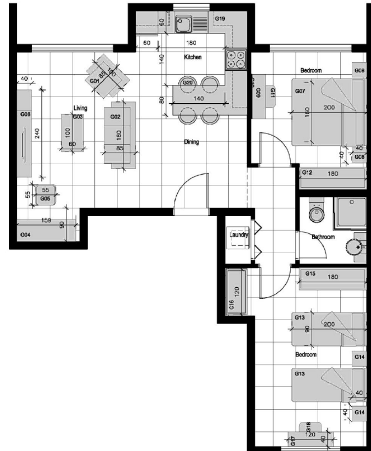
GROUND FLOOR PLAN - VILLA EXAMPLE
